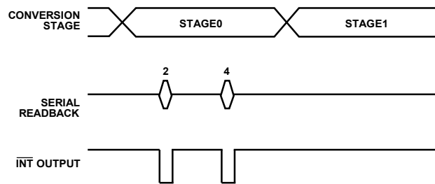
Figure 36. Example of Sensor Touch Interrupt
