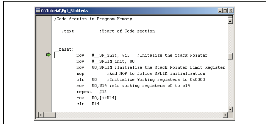
FIGURE 2-15: SOURCE CODE WINDOW
