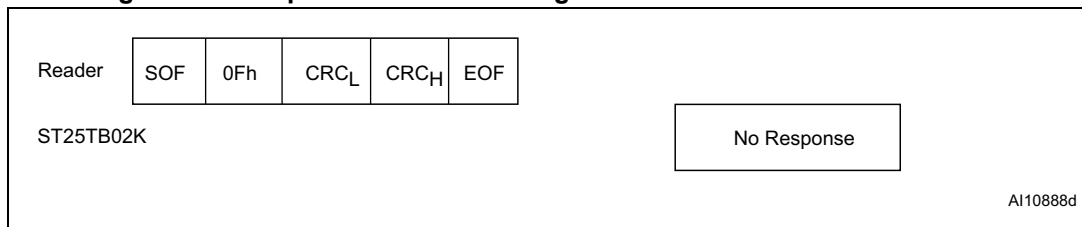
Figure 51. Completion frame exchange between reader and ST25TB02K
