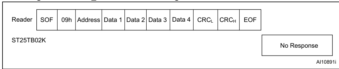
Figure 41. Write_block frame exchange between reader and ST25TB02K
