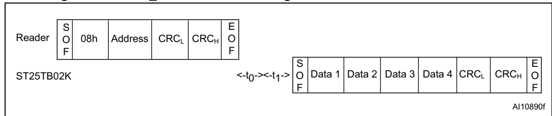
Figure 38. Read_block frame exchange between reader and ST25TB02K
