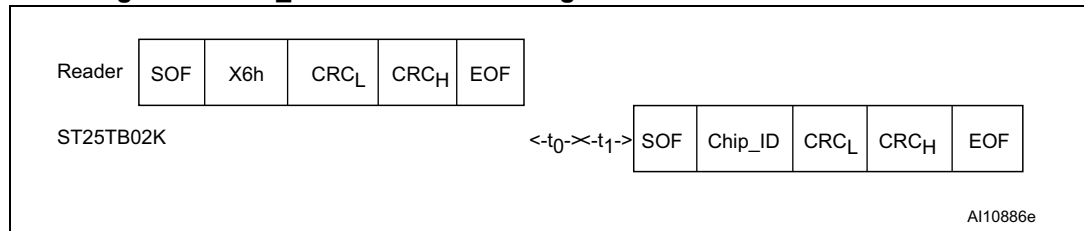
Figure 26. Slot_marker frame exchange between reader and ST25TB02K
