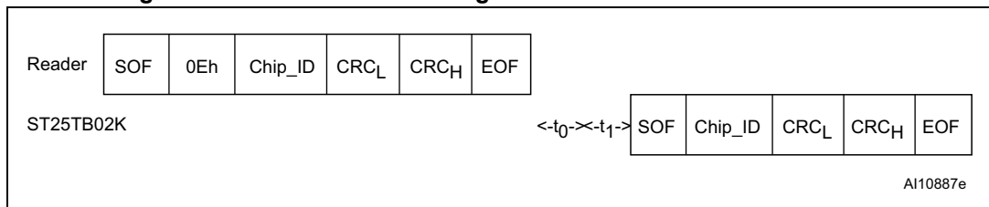
Figure 50. Select frame exchange between reader and ST25TB02K
