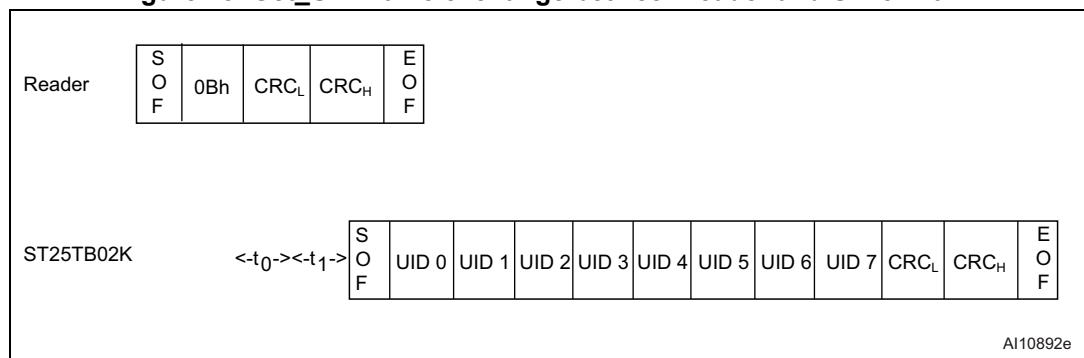
Figure 45. Get_UID frame exchange between reader and ST25TB02K
