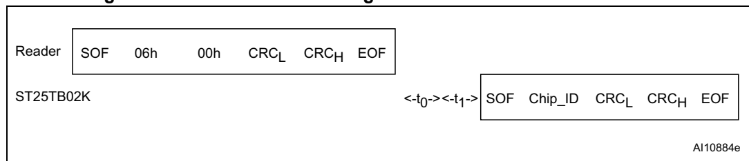
Figure 20. Initiate frame exchange between reader and ST25TB02K
