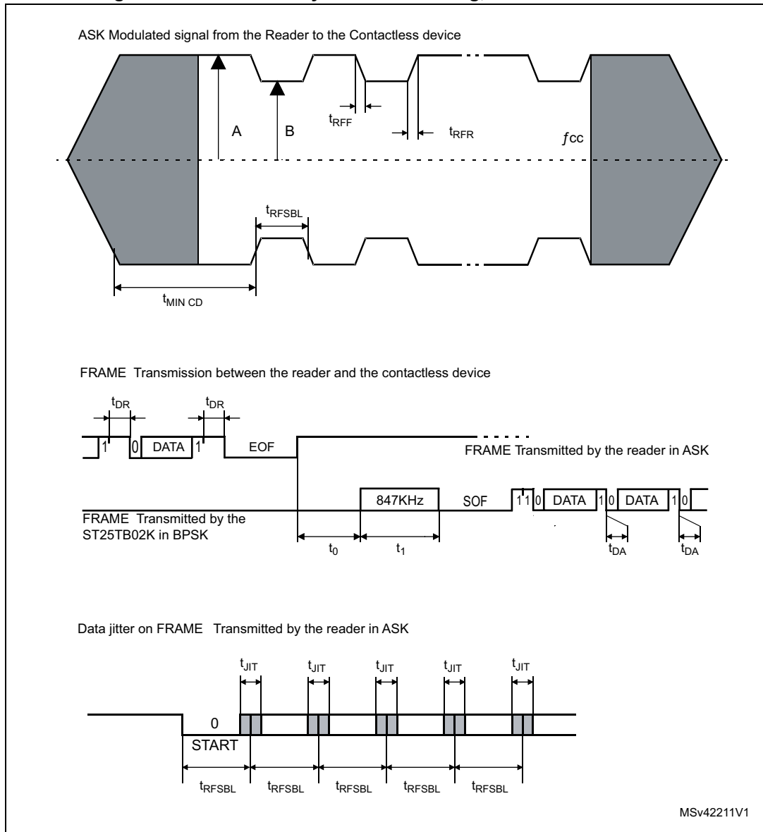
Figure 46. ST25TB02K synchronous timing, transmit and receive
