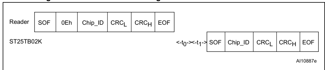
Figure 29. Select frame exchange between reader and ST25TB02K
