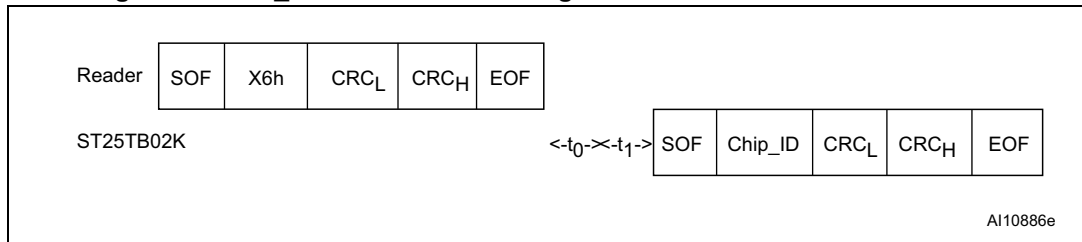
Figure 50. Select frame exchange between reader and ST25TB02K
