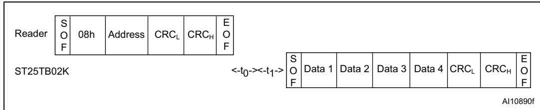
Figure 53. Read_block frame exchange between reader and ST25TB02K
