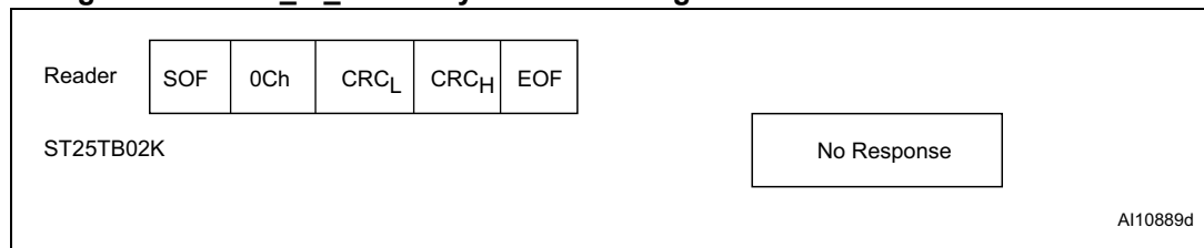
Figure 35. Reset_to_inventory frame exchange between reader and ST25TB02K
