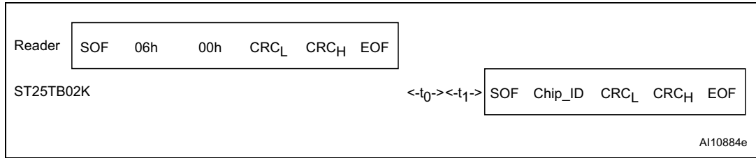
Figure 48. Pcall16 frame exchange between reader and ST25TB02K
