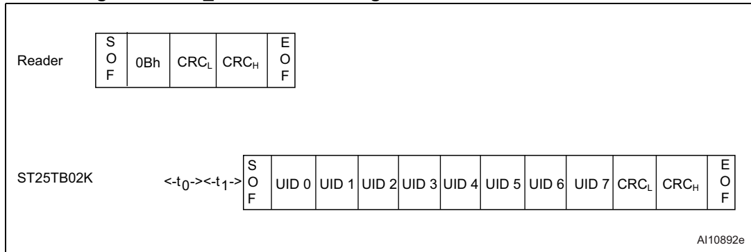
Figure 55. Get_UID frame exchange between reader and ST25TB02K
