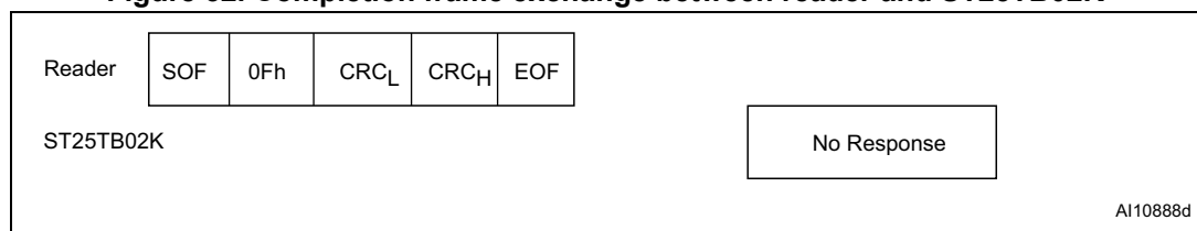
Figure 32. Completion frame exchange between reader and ST25TB02K
