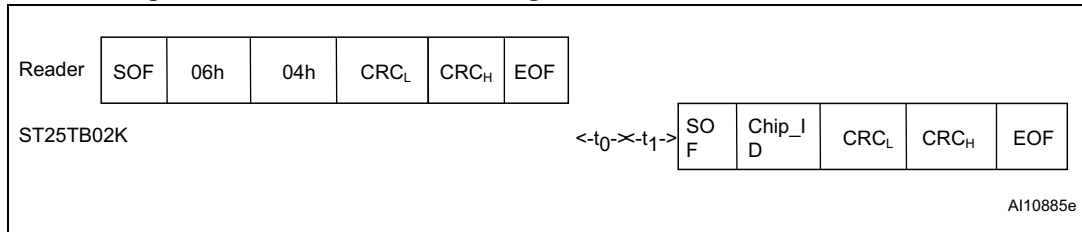
Figure 49. Slot_marker frame exchange between reader and ST25TB02K
