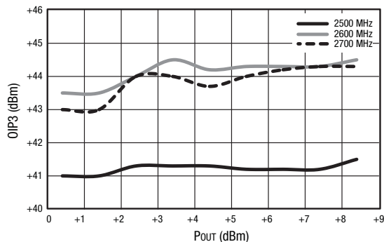
Figure 68. OIP3 vs Pout @ 2700 MHz
