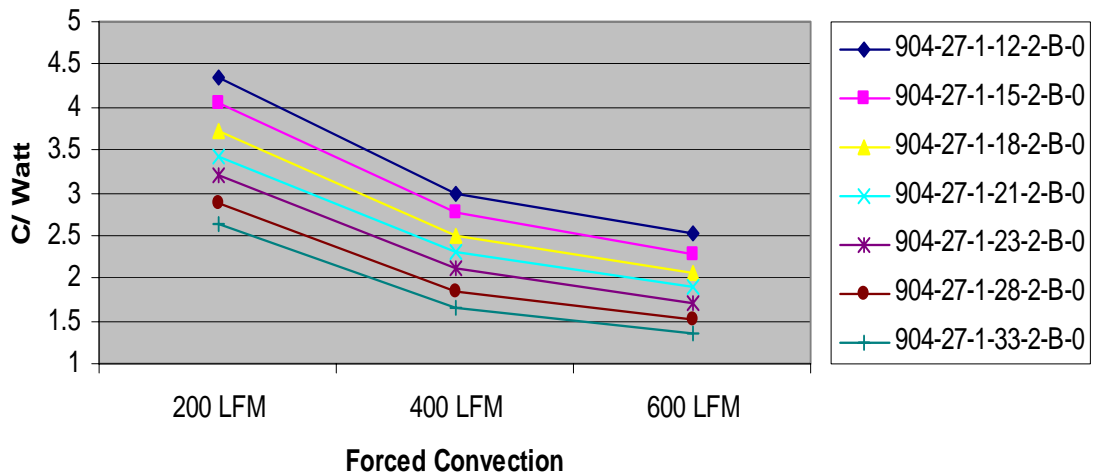
Thermal Performance
