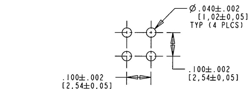
P.C. BOARD HOLE PATTERN
